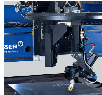
The plasma bevel cutting unit Skew Rotator Infinity facilitates the immediate cutting of bevels on parts
