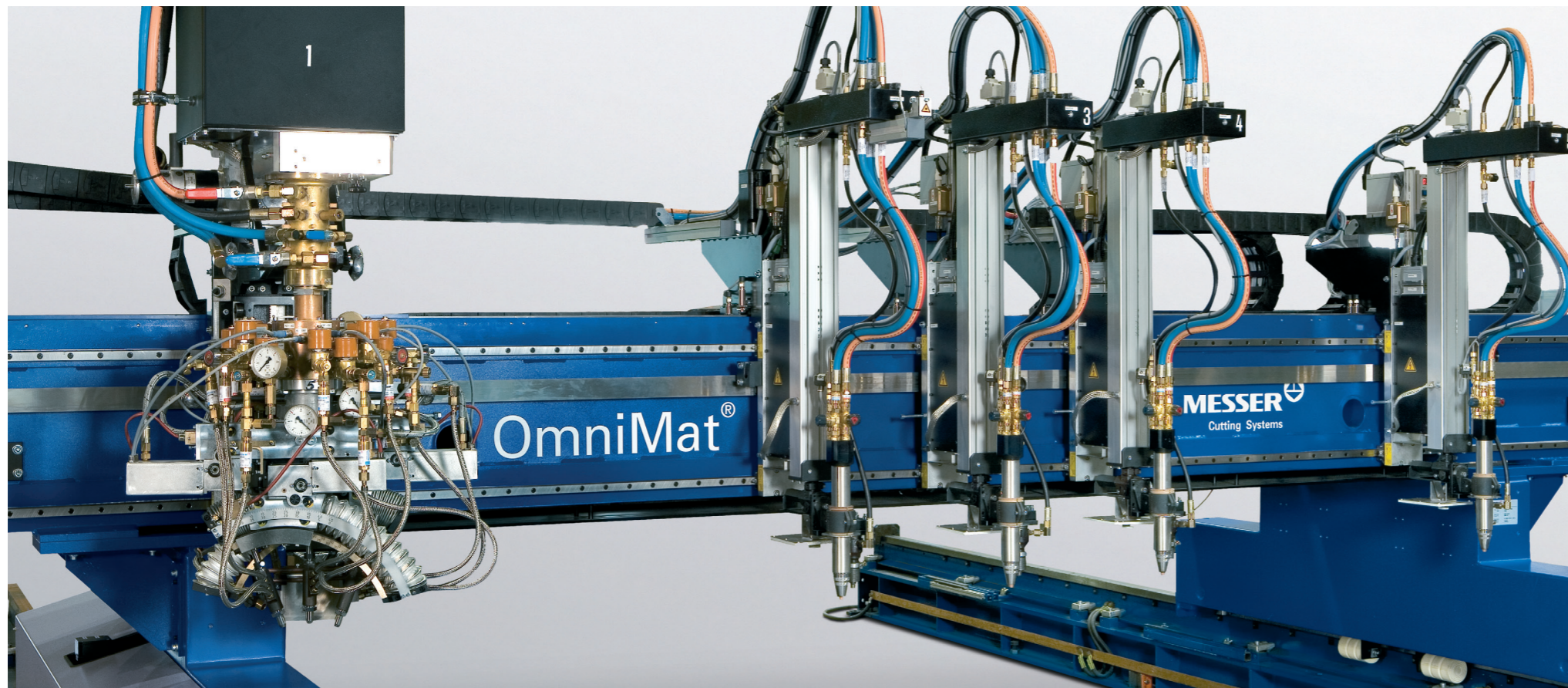
The plasma bevel cutting unit Skew Rotator Infinity facilitates the immediate cutting of bevels on parts
